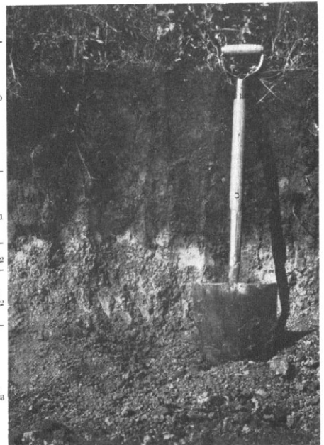
Fig. 2. —Profile of Peace Hills fine sandy loam. Note the deep A_1 horizon (18"). This soil will erode with the wind unless the organic matter content of the surface soil is maintained.
