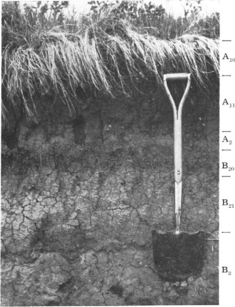
Fig. 3.—A profile of Beaverhills loam. It is the (normal) prismatic-chnozem profile. It usually occurs nearer to the hill tops than the Angus Ridge loam. The depth of black A 1 varies considerably; some of the hill tops may be quite thin.
