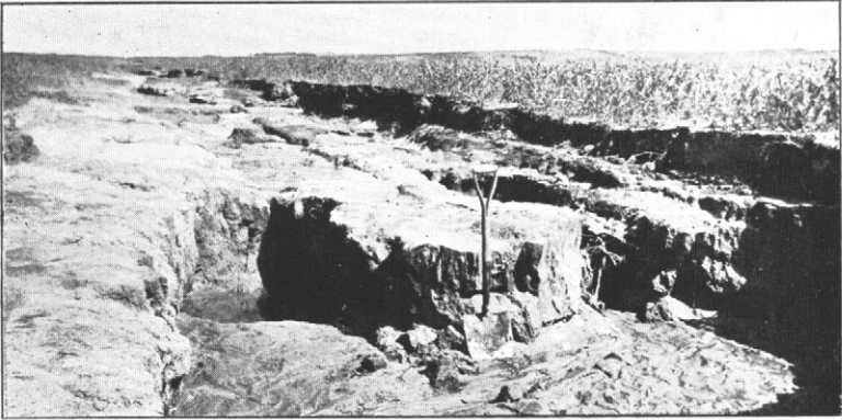
Fig. 1. —Water erosion on Killam loam. A heavy downpour or spring runoff may wash away the entire A_1 horizon. (See Plate VII, fig. 2).
