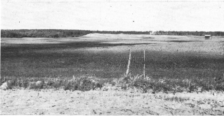
Fig. 1.—An area of mixed Falun and Breton soil types. The greyer Breton soil is usually confined to the higher land in these mixed areas.
