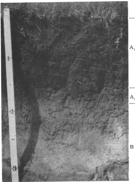
Fig. 3. —Profile of Ponoka loam. Note the deep black A_1 horizon and the thin A_2 horizon. This is a solodic profile. Usually the underlying glacial till is found within three to five feet of the surface.
