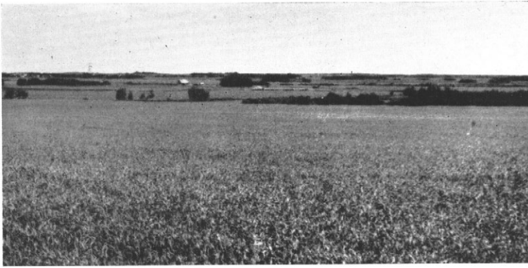
Fig. 1. —The level alluvial plain at New Norway. This is primarily a mixture of Ponoka loam and Peace Hills fine sandy loam. Angus Ridge loam occurs where the underlying till comes to the surface. It is good arable land.
