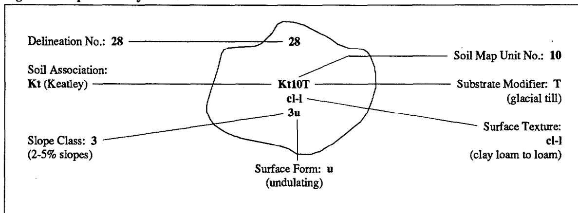
Figure 1. Sequence of Symbols.
